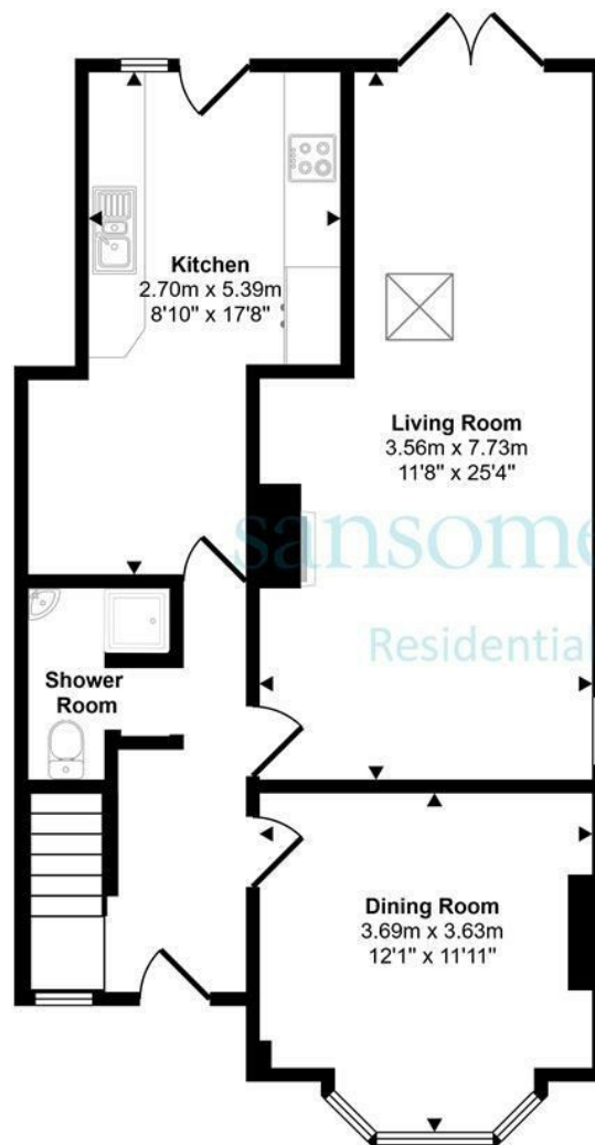
Ground Floor Approx 64 sq m / 686 sq ft
